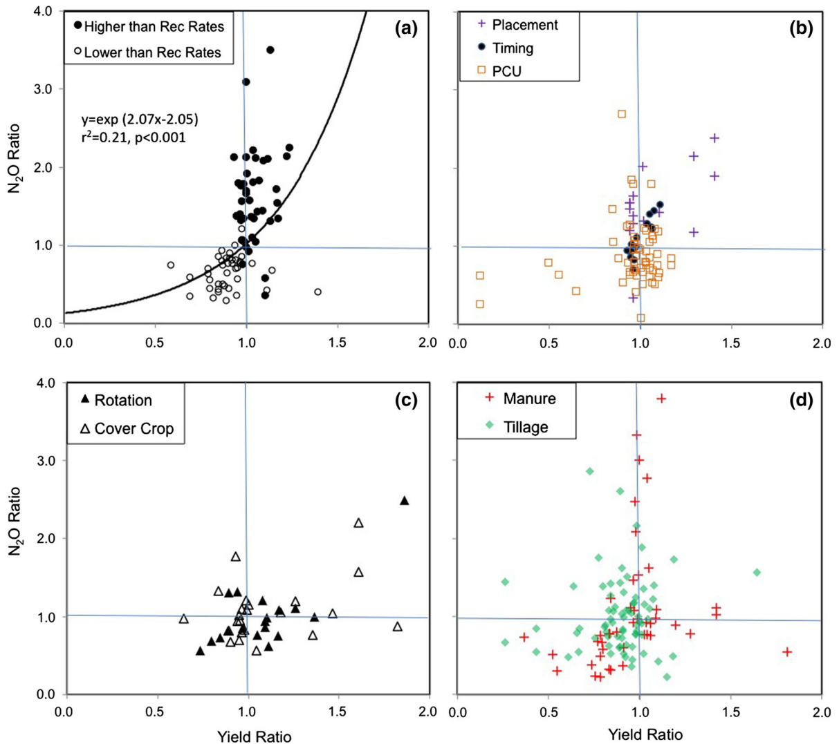
Fig. 5 The tradeoff between yield and N_2O mitigation. The Yield Ratio (X-axis) is calculated as the ratio of treatment yields to control yields and the N_2O ratio (Y-axis) is treatment N_2O emissions from over those from the controls. To increase the clarity of the graphs, some data points with extreme values were not shown. Seven data points in the Tillage group reporting a yield ratio larger than 2.0 and N_2O ratios of 0.56–1.8 are not
